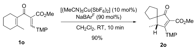
Scheme 4. Copper-mediated cyclization of 1,4-dien-3-one 1o .
