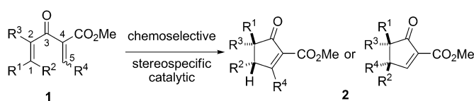
Scheme 2. The challenge: selectivity in cyclopentenone synthesis.
